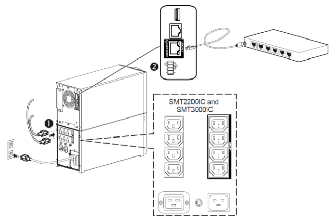
SMT2200C, SMT2200IC, SMT3000C and SMT3000IC Tower Models
