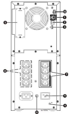
SMT2200IC and SMT3000IC Tower
