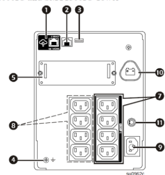
SMT1000IC and SMT1500IC Tower
