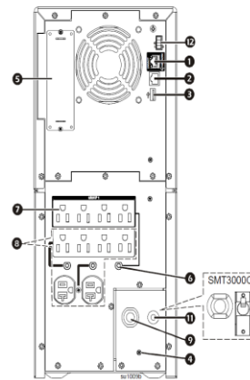
SMT2200C and SMT3000C Tower
